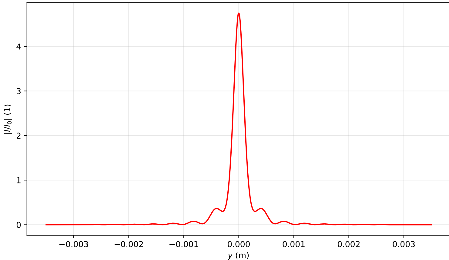
Intensity profile I(x=0, y, z=0.318)/I_0 , \text{Pin}=1.0\text{Pcr} , artificial time
